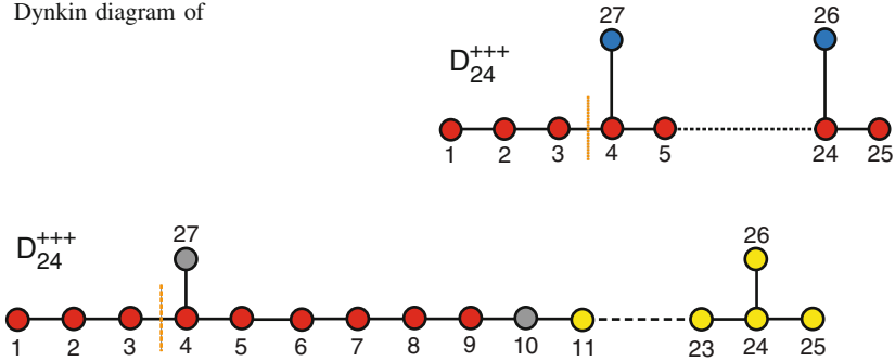
Fig. 7 The decomposition of D_{24}^{+++} into A_9 \times D_{16} with levels defined by the nodes \alpha_{27} and \alpha_{10}
