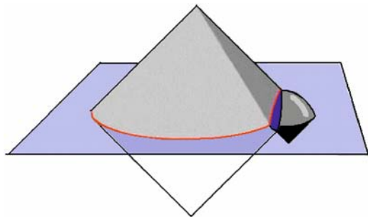
Fig. 14 A bubble of True vacuum forms in the Black false vacuum and then collides with a bubble of White vacuum. The true vacuum is bounded by a hat but the White vacuum terminates in a space-like surface. Some generators of the hat intersect the Black vacuum and some intersect the White. Thus \Sigma , shown as the red curve, is composed of two regions
