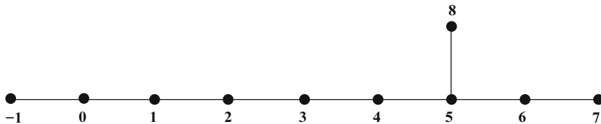
Fig. 2 The hyperbolic algebra E_{10} . The nodes labelled 1, ..., 8 form the Dynkin diagram of E_8 , the nodes 0, 1, ..., 8 form the Dynkin diagram of its affine extension E_8^+ , while the nodes -1, 0, 1, \dots, 8 define its overextension E_8^{++} \equiv E_{10}
