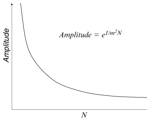
Fig. 3 No boundary amplitude
