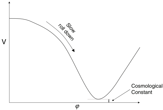
Fig. 2 New inflationary scenario
